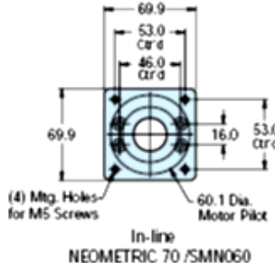
Part No. 002-3616-01 NEOMETRIC 70 / SMN060
