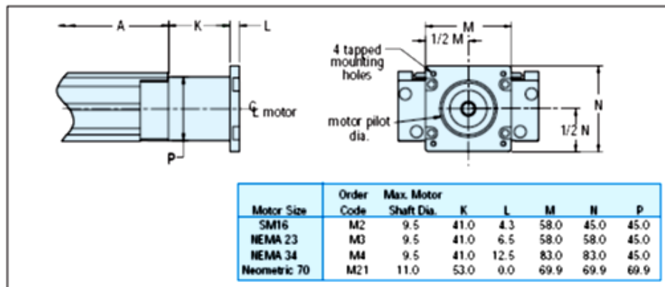
Part No. 002-3615-01 NEMA 23
