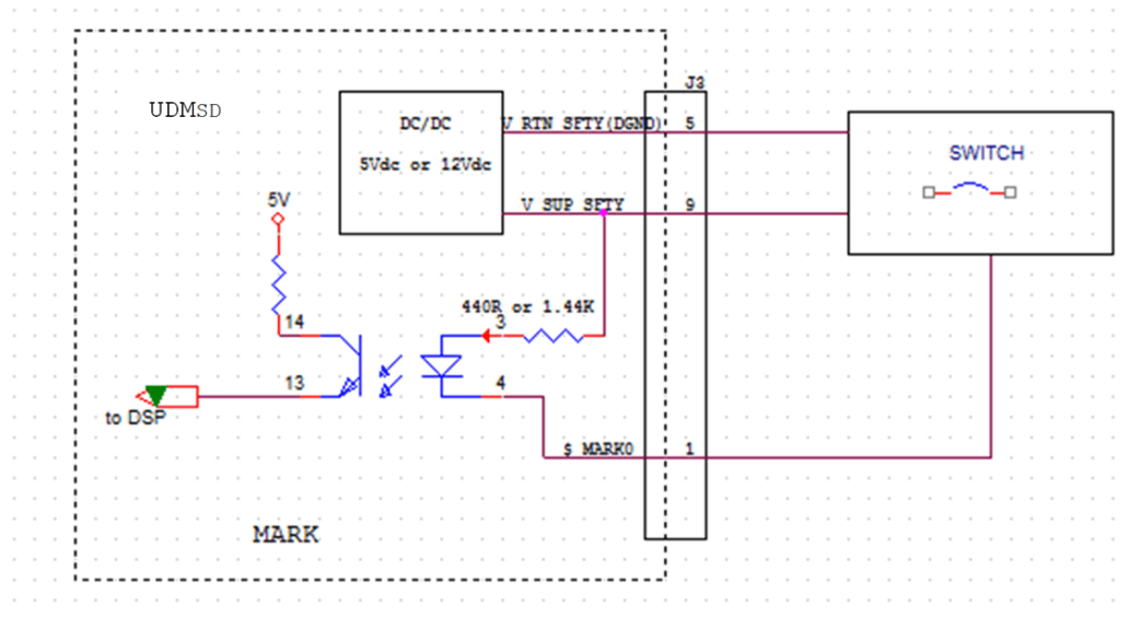
Figure 10-1. MARK inputs
