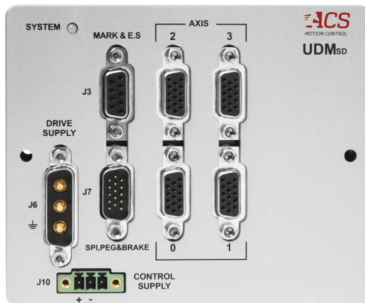
Figure 20-1. UDMsd Connectors
