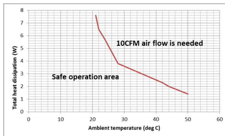
Figure 15-2. Thermal Considerations Chart B
