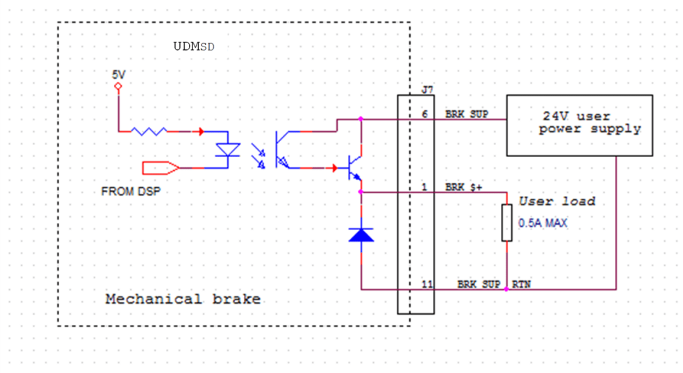
Figure 6-1. Mechanical Brake
