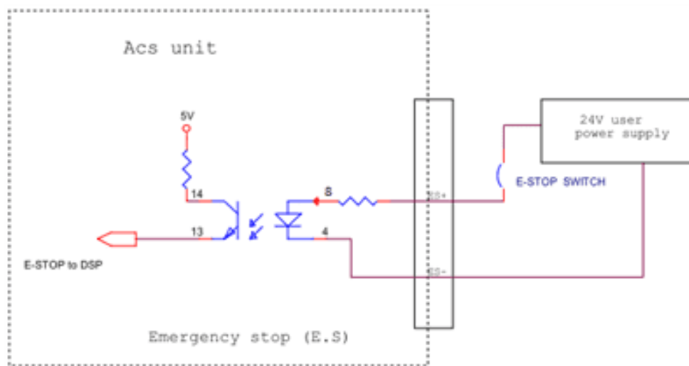
Figure 11-1. Emergency Stop Input
