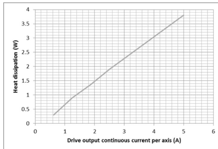
Figure 15-1. Thermal Considerations Chart A
