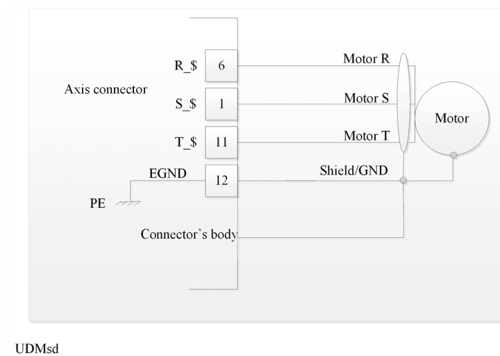
Figure 4-2. 3-Phase Motor Connection
