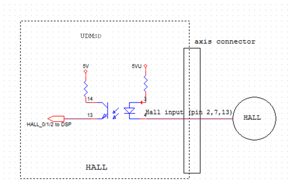
Figure 9-1. HALL Sensor Connection
