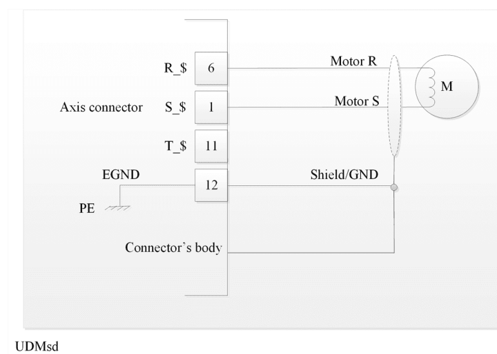
Figure 4-3. DC Brush Motor Connection
