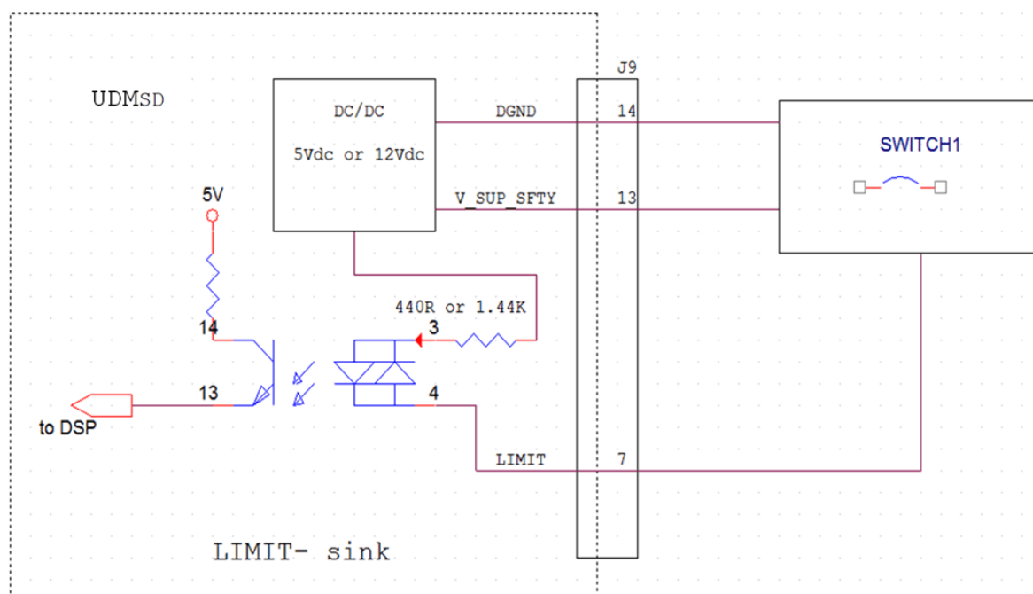
Figure 12-1. R/L Limit Connections
