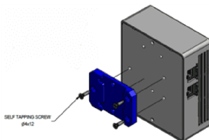
Figure 17-3. DIN rail mounting
