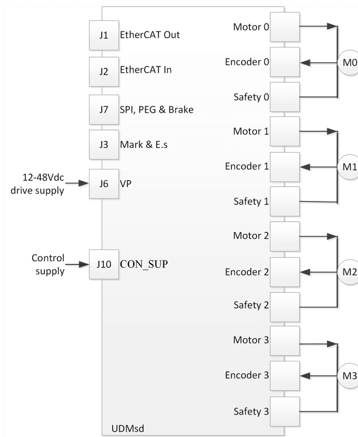
Figure 4-1. UDMsD Connection Schematic
