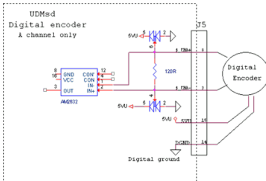
Figure 7-1. Incremental Digital AqB Encoder Connections
