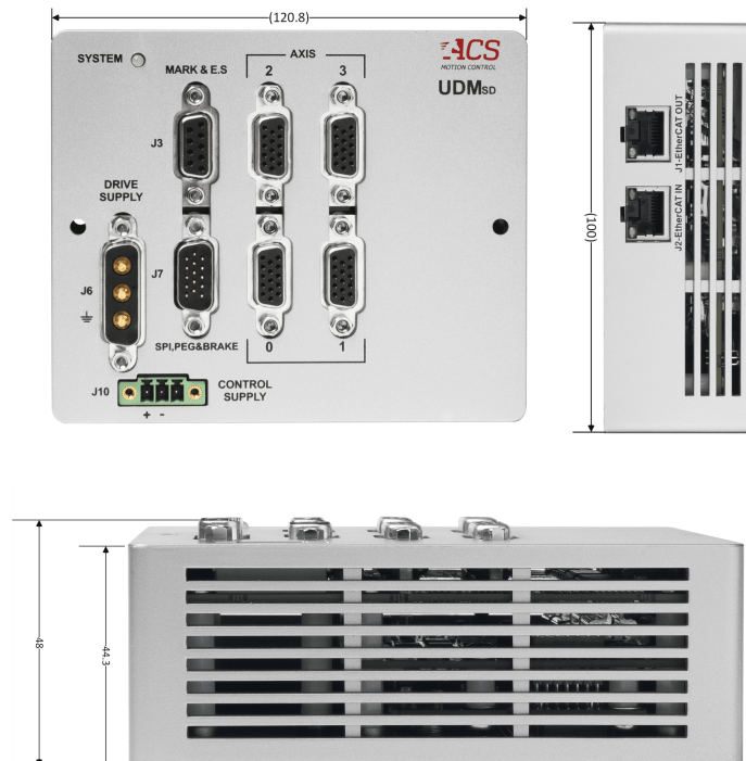
Figure 17-1. External Dimensions
