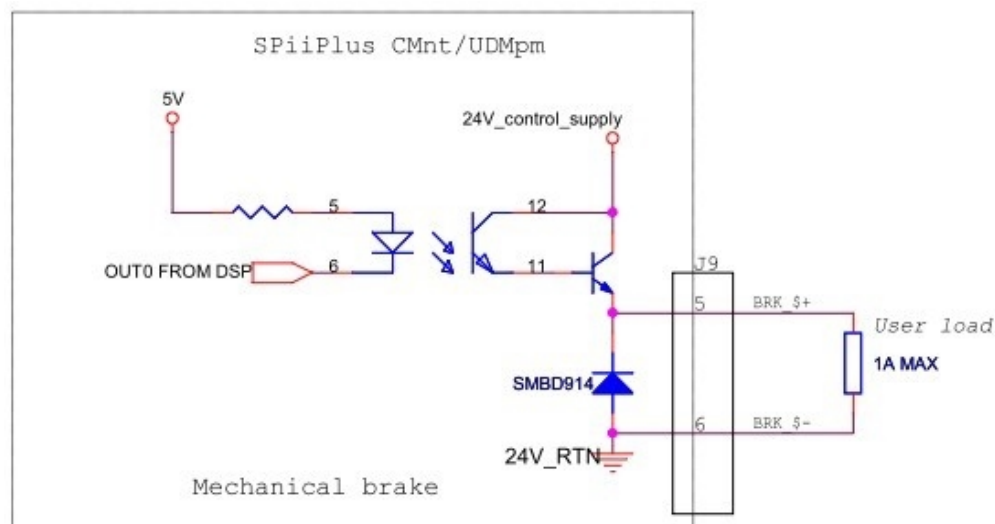
Figure 4-23. Mechanical brake
