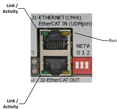
Figure 2-6. EtherCAT indicators
