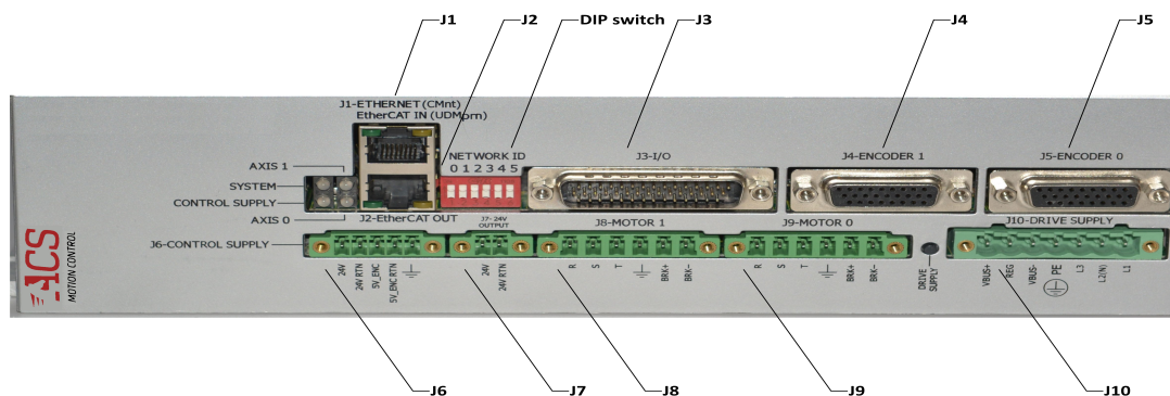
Figure 2-1. Front view - connectors and DIP switch
