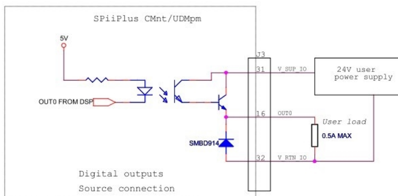
Figure 4-8. Digital output connections
