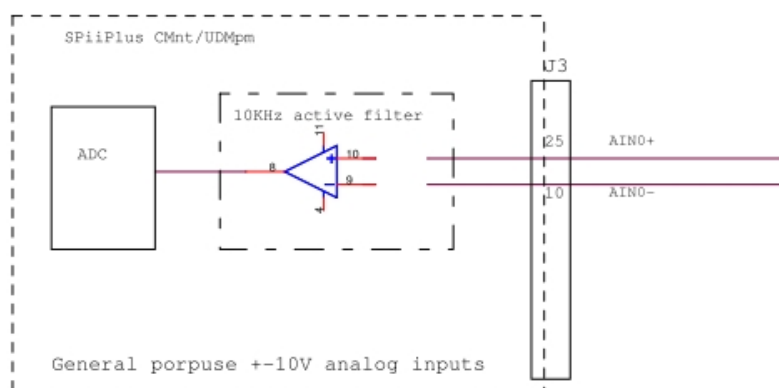
Figure 4-4. General purpose analog inputs
