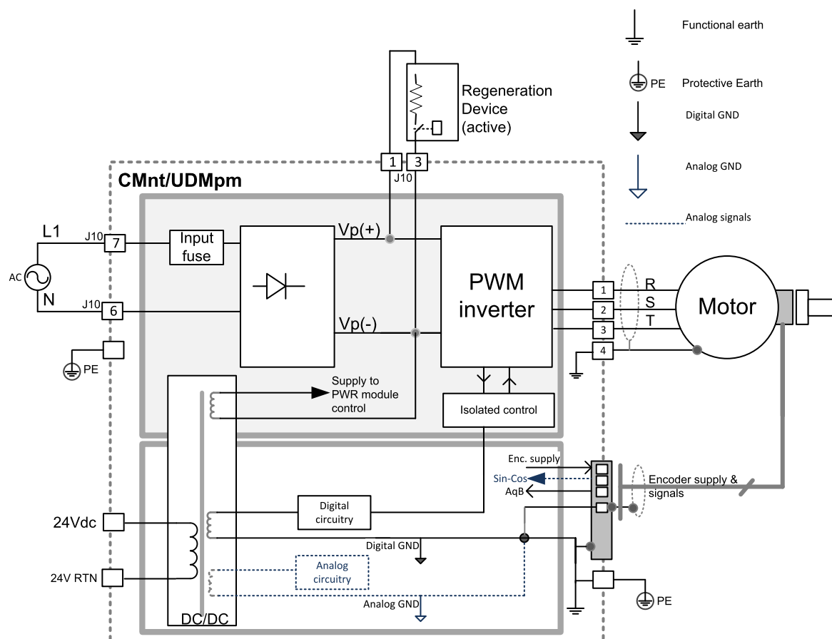
Figure 4-1. Grounding and shielding
