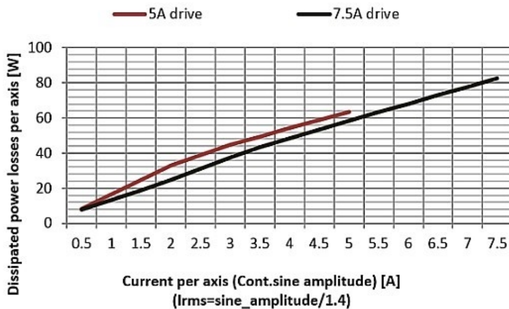
Figure 5-4. Dissipated power vs current
