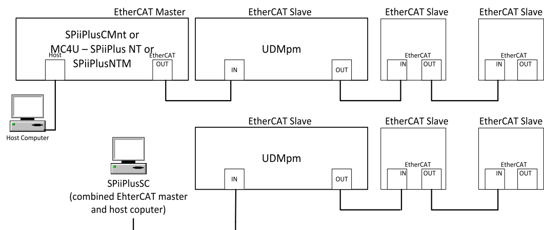
Figure 5-2. EtherCAT network connections
