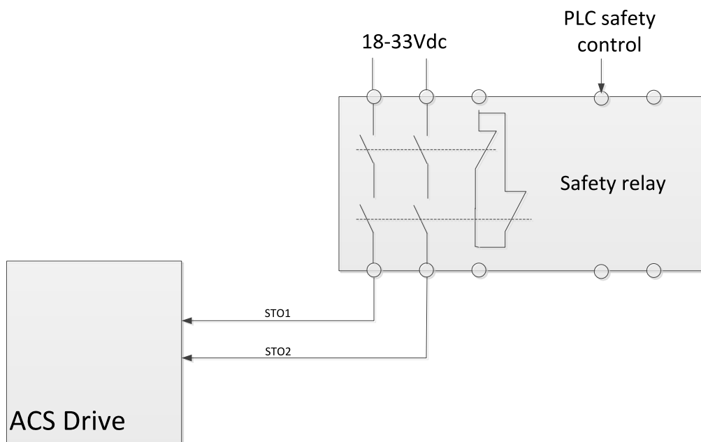
Figure 4-9. STO wiring scheme
