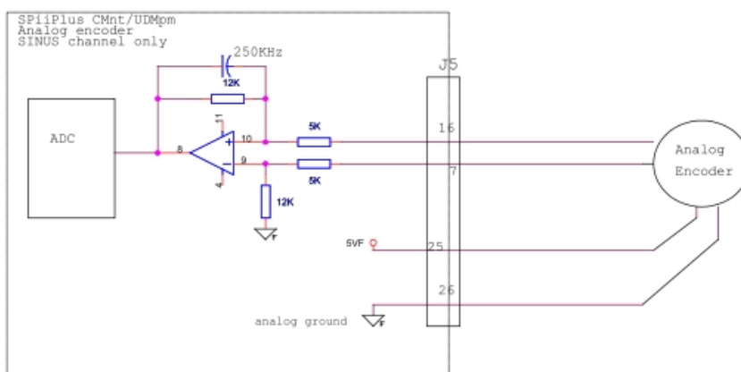
Figure 4-13. Sin-Cos encoder connections
