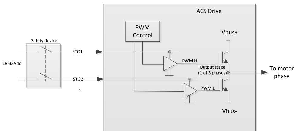
Figure 4-10. STO implementation
