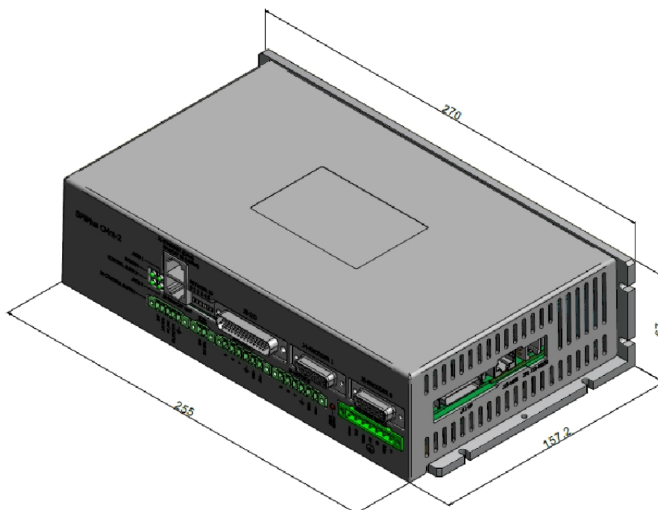
Figure 5-3. UDMpm dimensions
