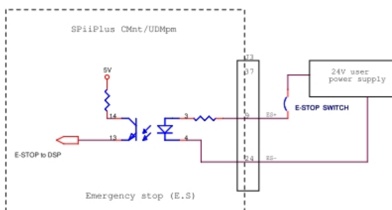
Figure 4-6. Emergency stop input
