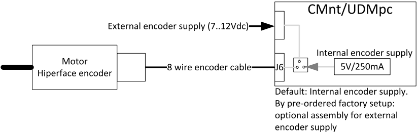
Figure 4-17. External power connection
