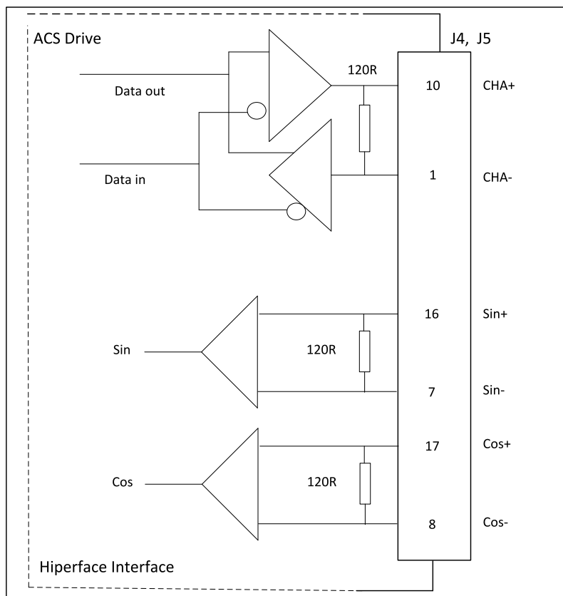
Figure 4-14. Absolute encoder hipurface schematic diagram
