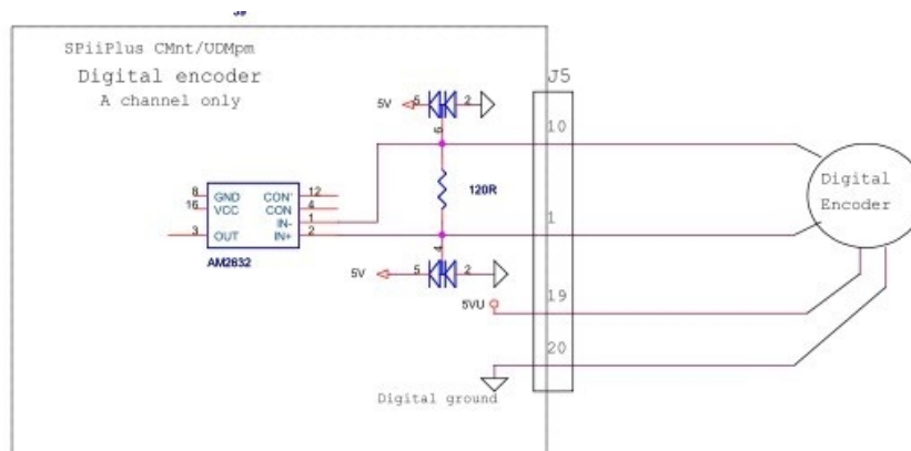
Figure 4-11. Incremental digital AqB encoder connections
