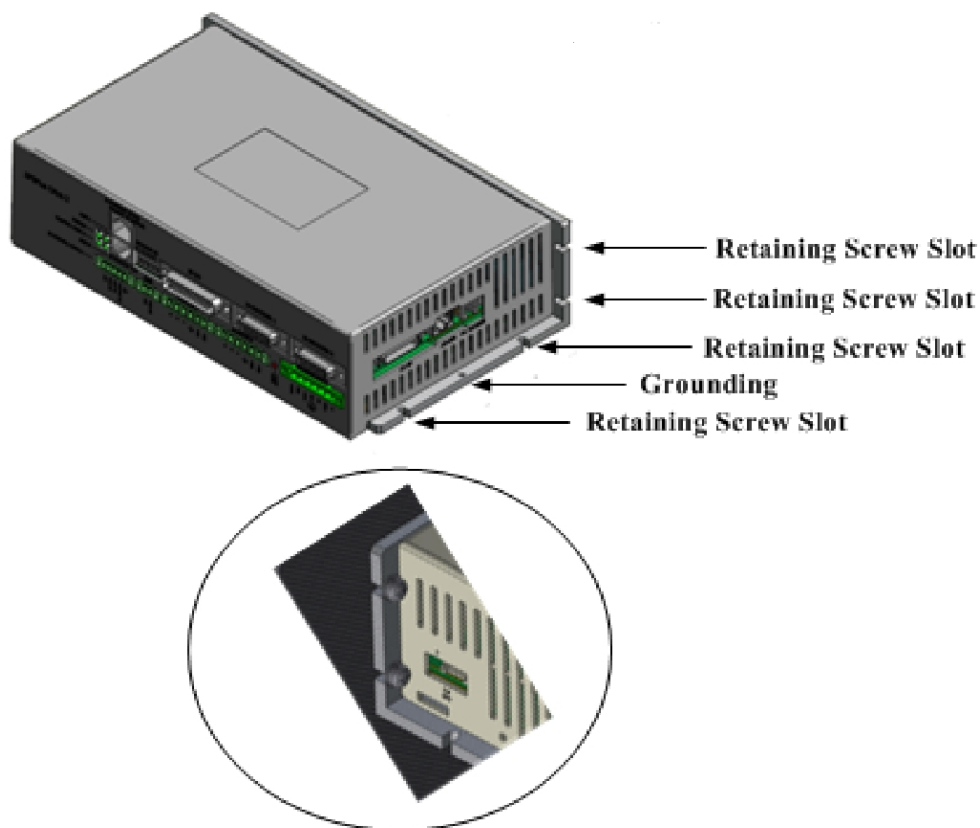
Figure 3-1. Retaining screw locations
