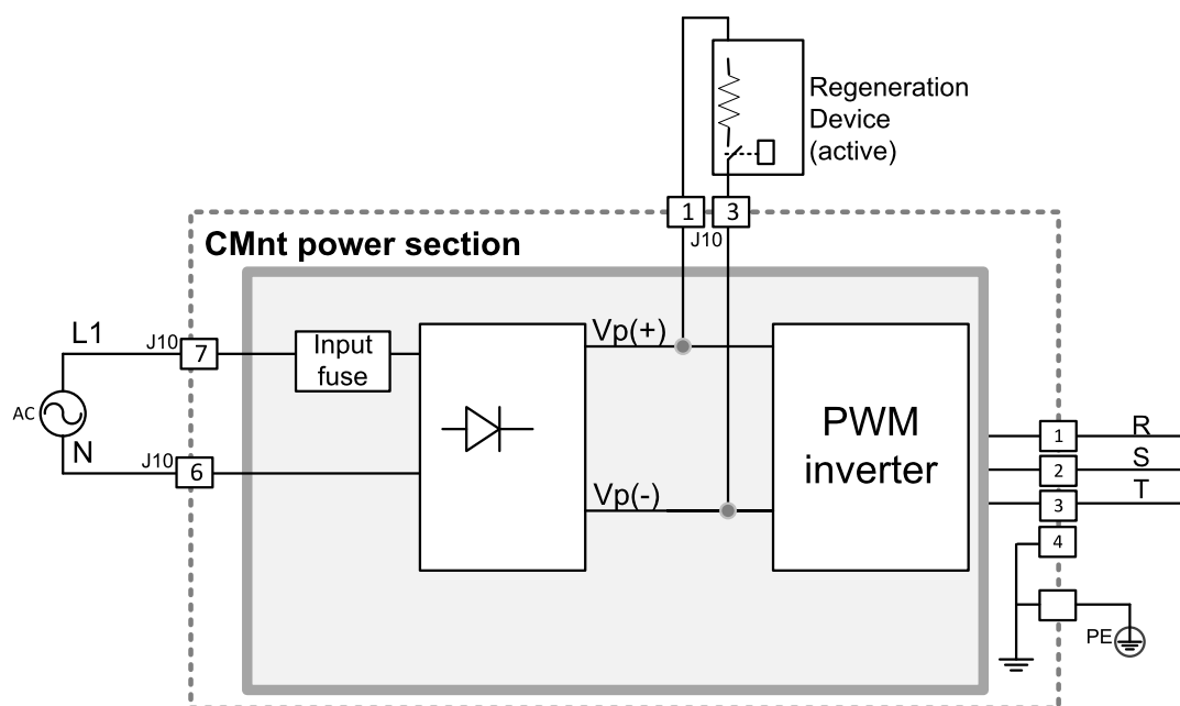
Figure 5-1. Regeneration connection
