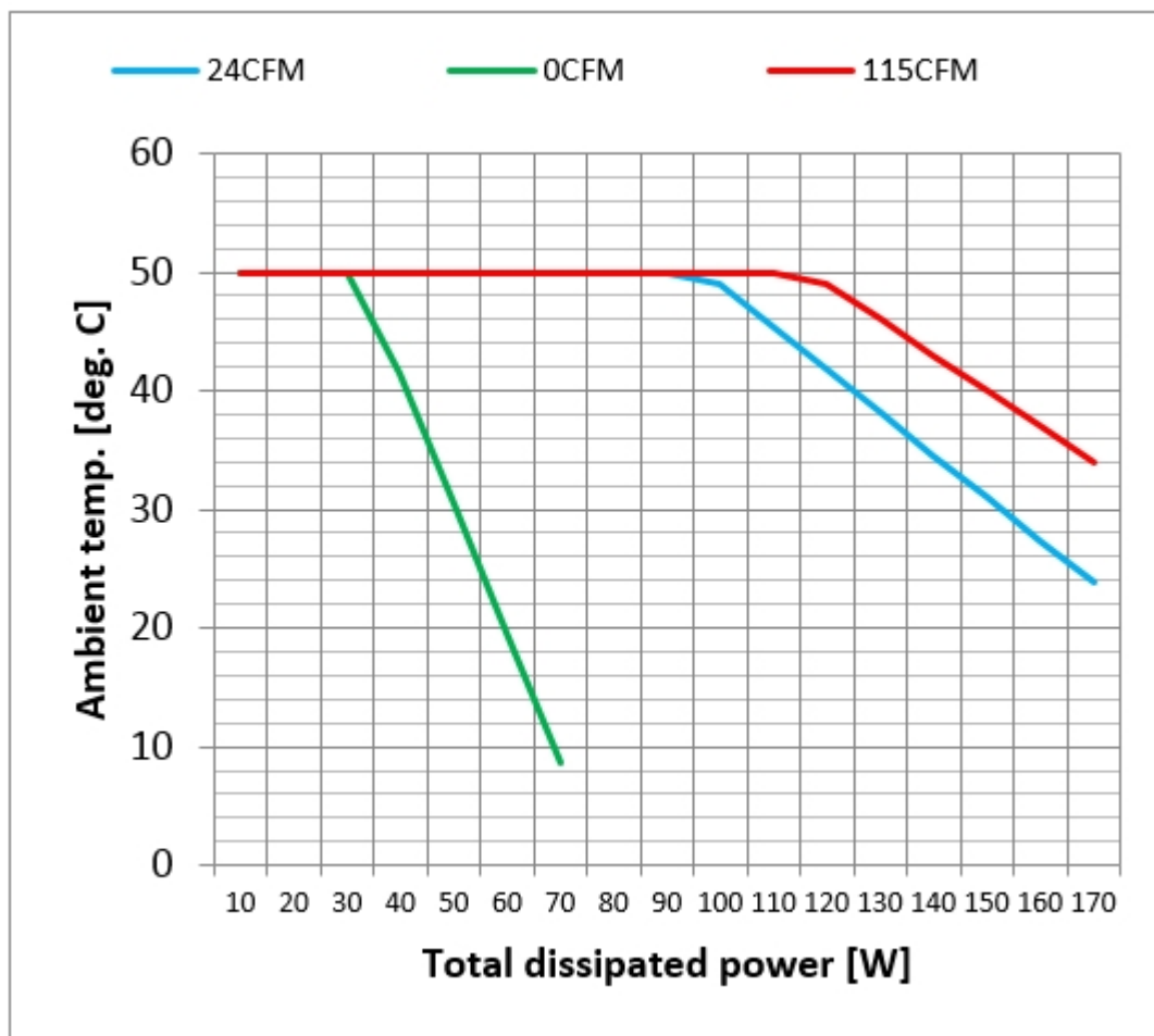
Figure 5-5. Dissipated power vs temperature
