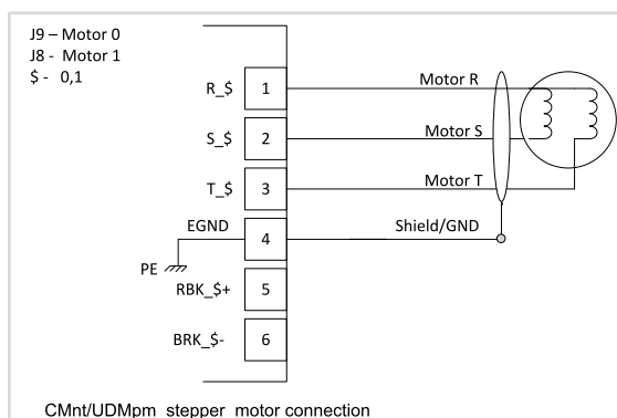
Figure 4-20. Two-phase motor connection
