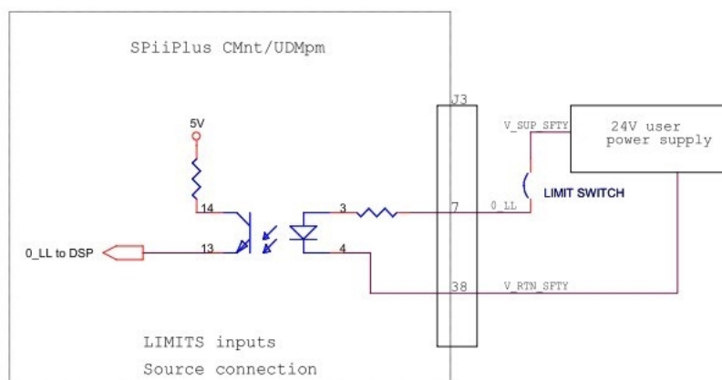
Figure 4-5. Limit connections
