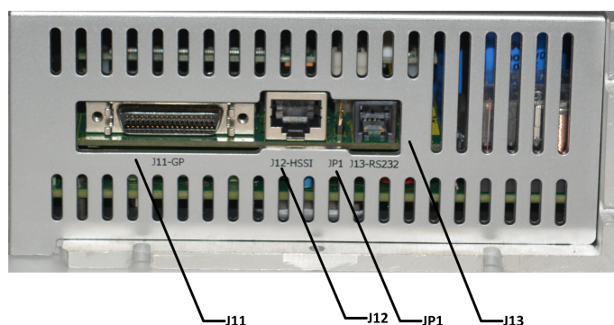
Figure 2-2. Right side view - connectors and jumper
