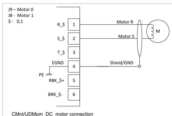
Figure 4-19. DC brush motor connection
