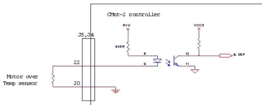
Figure 4-21. Motor over temperature connection
