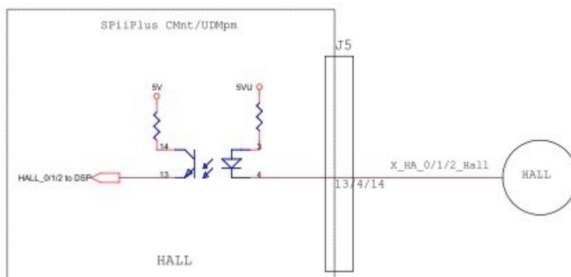
Figure 4-12. Hall sensors connection
