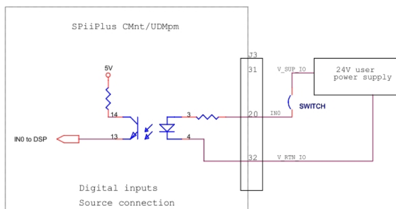
Figure 4-7. Digital input connections
