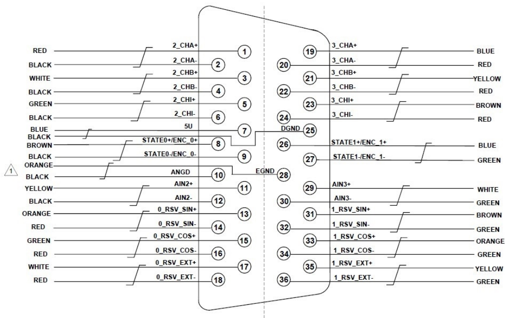
Figure 2-7. Cable kit
