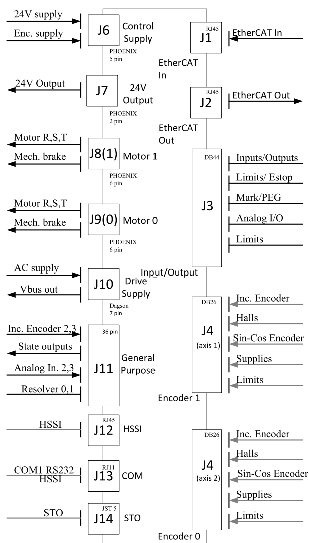
Figure 1-1. Interface block diagram
