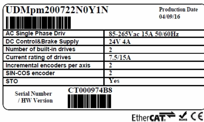
Figure 2-9. Label with ordered P/N example
