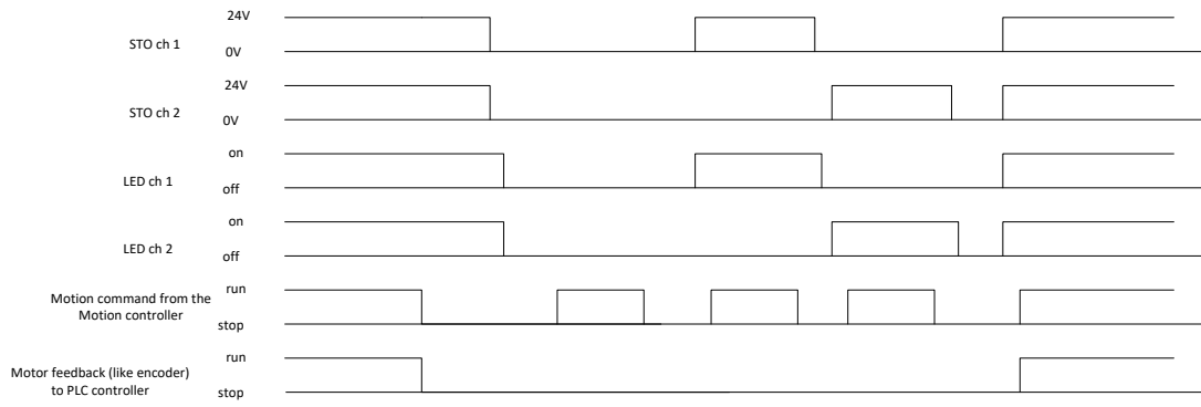
Figure 7: J2 signals and its LEDs
