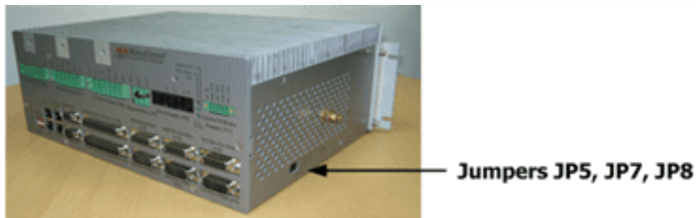
Figure 9-7. Jumper Locations
