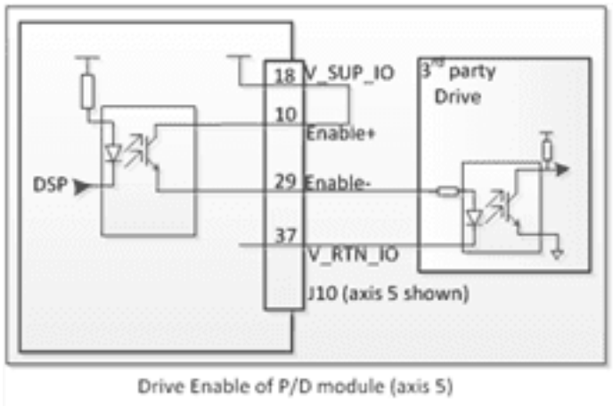
Figure 4-5. Drive Enable of P/D module (axis 5)
