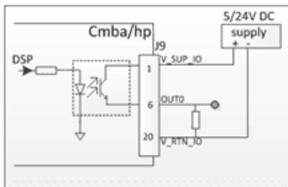
Figure 7-1. Digital Output Connection (source)
