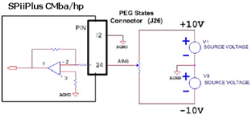
Figure 8-2. Single-axis Joystick Through AIN6
