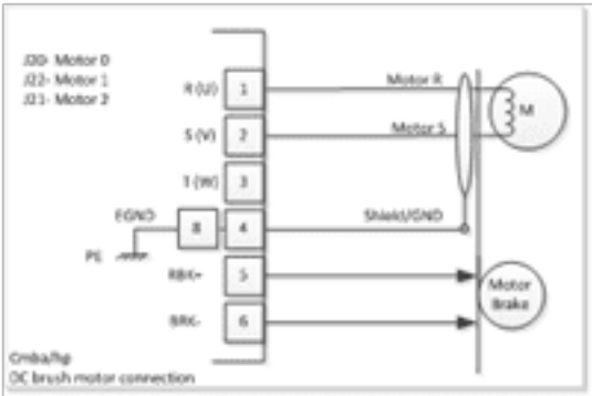
Figure 3-2. DC Brush Motor Connection
