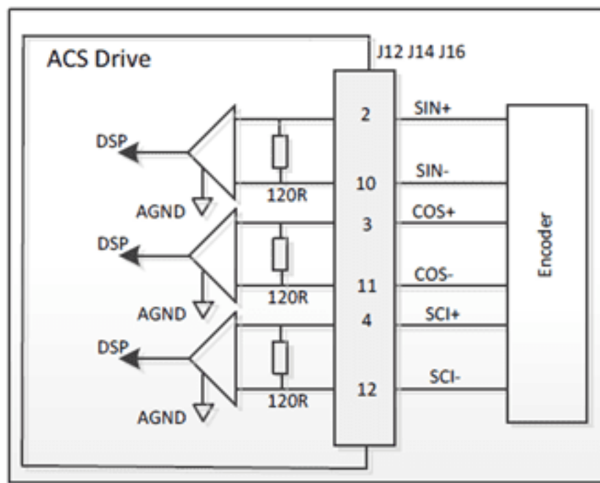
Figure 4-2. Sin-Cos Encoder Connections
