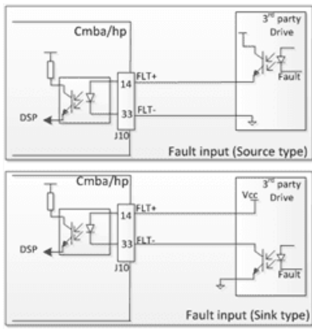
Figure 4-6. Fault signal electrical schematic, 'source' and 'sink' connectivity scheme.
