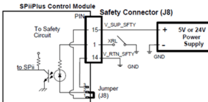
Figure 9-2. Right Limit (Sink) schematic diagram
