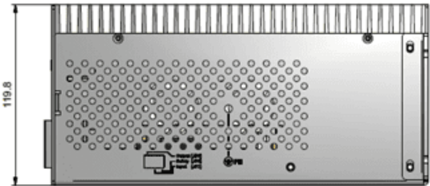
Figure 14-4. SPiiPlusCMHP/BA Rear
