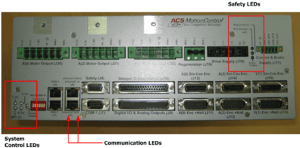
Figure 9-6. SPIIPlusCMHP/BA LED Indicators
