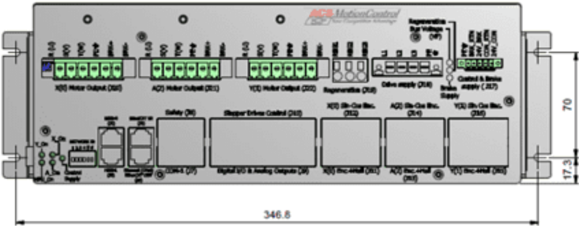
Figure 14-1. SPiiPlusCMHP/BA Front
