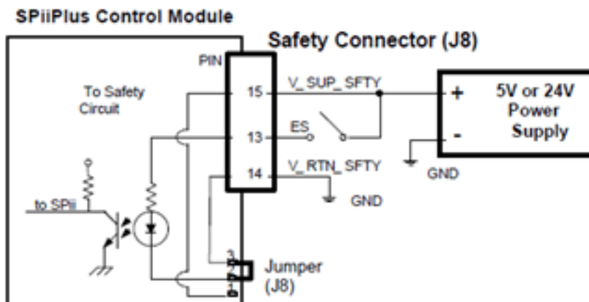
Figure 9-3. Emergency Stop Source Input
