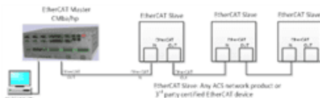
Figure 10-1. CMHP/BA as master with 3rd party drives as slaves in an EtherCAT network
