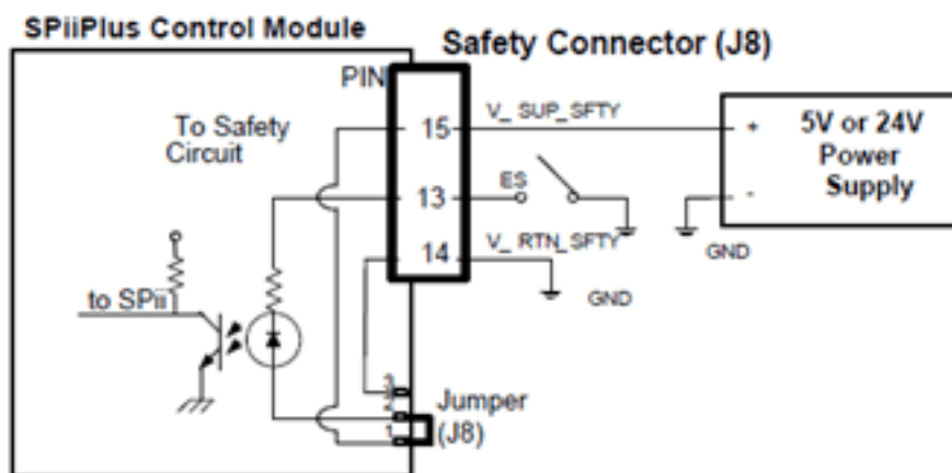
Figure 9-4. Emergency Stop (Sink) schematic diagram
