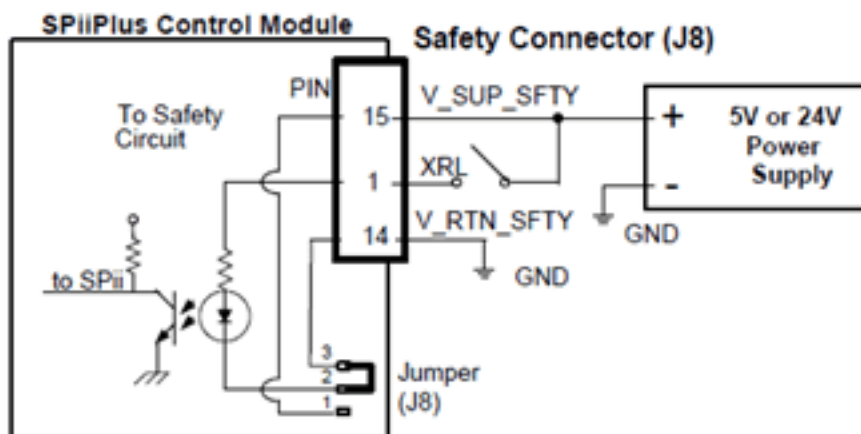
Figure 9-1. Right Limit (Source) schematic diagram
