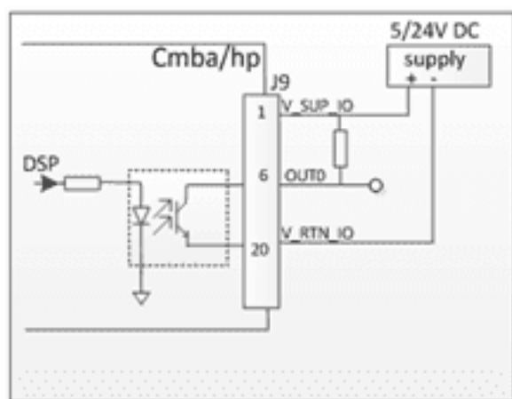
Figure 7-2. Digital Output Connection (sink)
