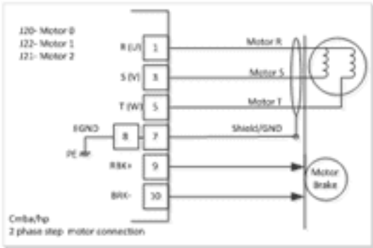
Figure 3-3. 2-Phase Step Motor Connection
