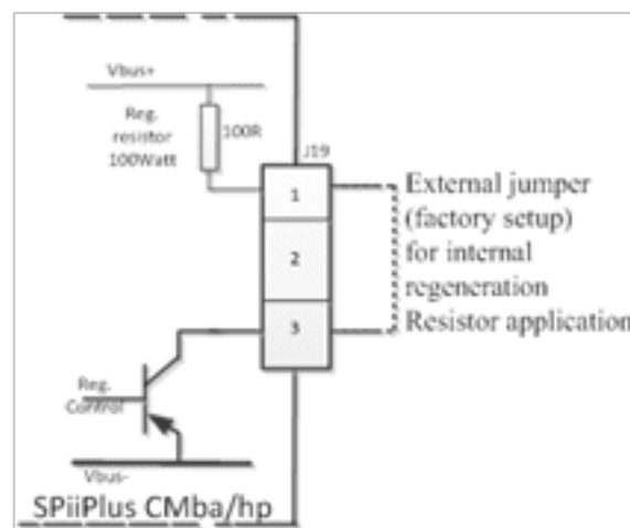
Figure 3-5. Internal Regeneration Connection
