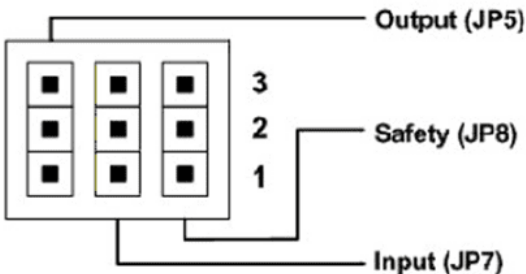
Figure 9-8. Sink or Source Jumper Configuration
