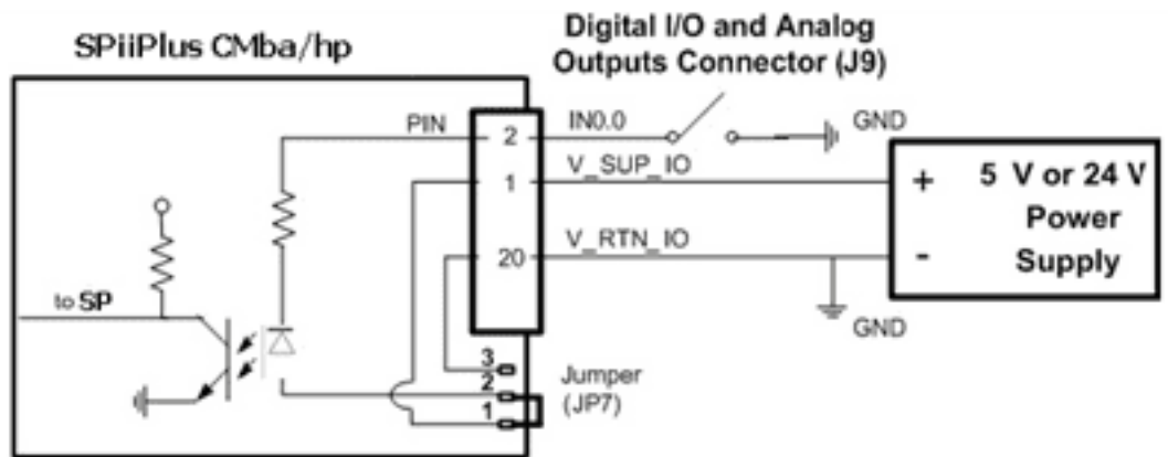
Figure 7-3. Source Digital Inputs
