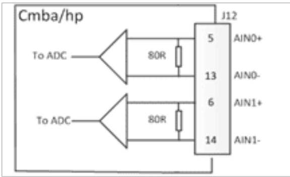
Figure 8-1. General Purpose Analog Inputs
