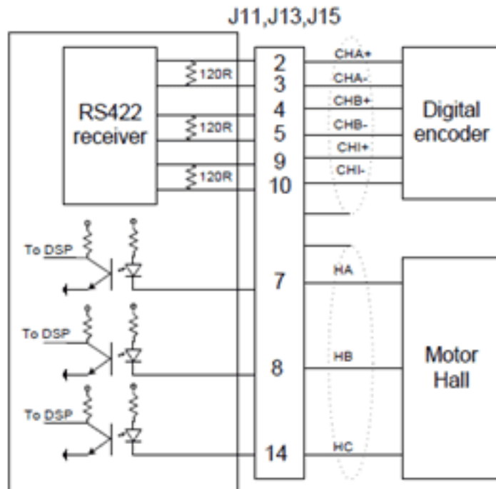
Figure 4-1. Incremental Digital AqB Encoder Connections
