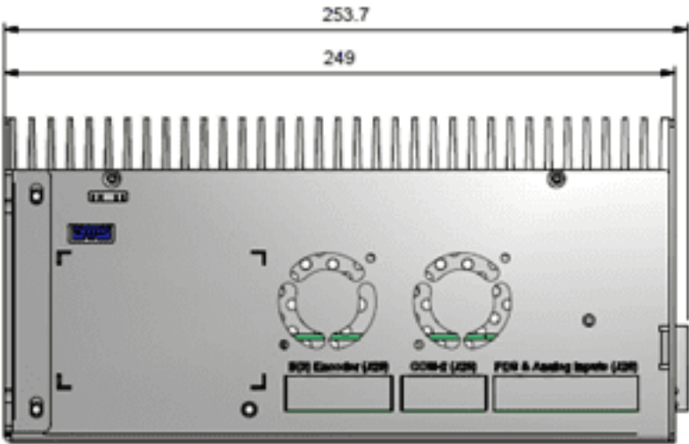
Figure 14-2. SPiiPlusCMHP/BA Side
