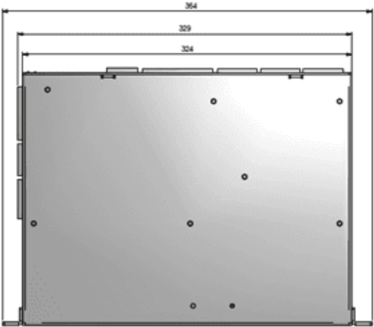
Figure 14-3. SPiiPlusCMHP/BA Bottom
