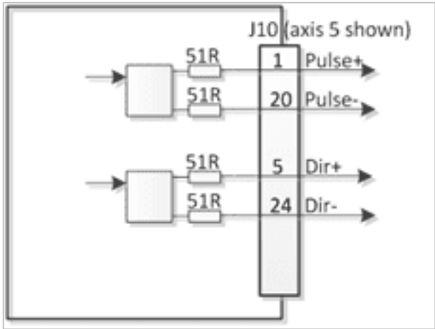
Figure 4-4. Pulse and Direction electrical schematic
