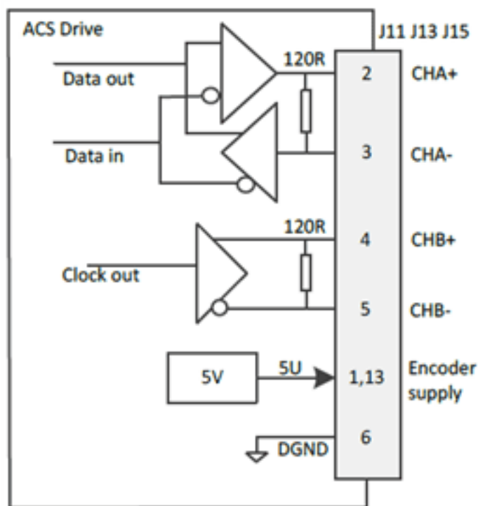
Figure 4-3. Absolute Encoder Connection
