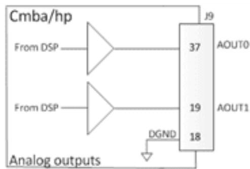
Figure 8-3. Analog output schematic diagram
