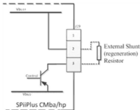
Figure 3-6. External Regeneration Connection
