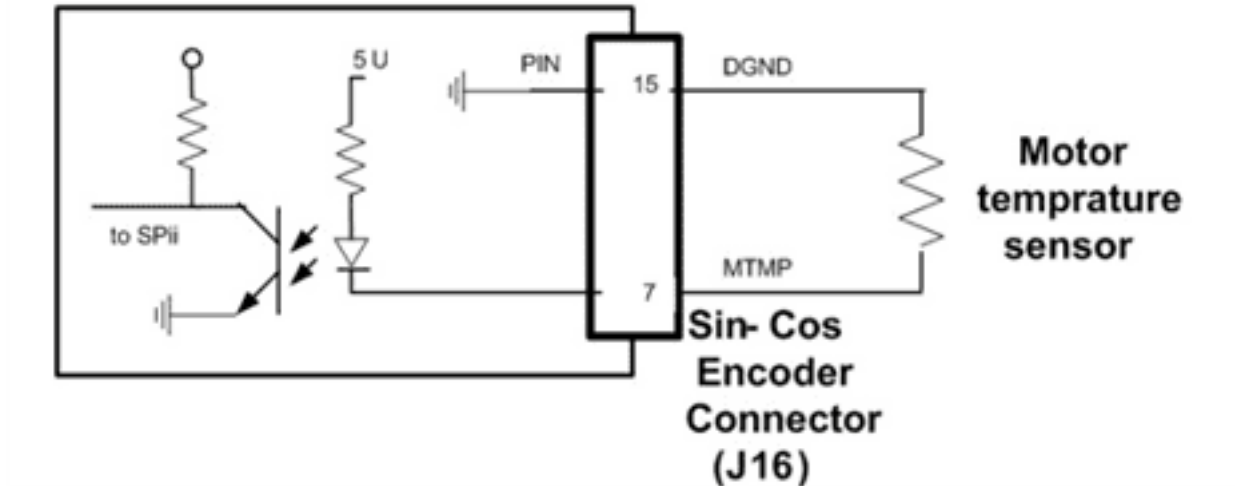
Figure 9-5. Motor Over Temperature Connection
