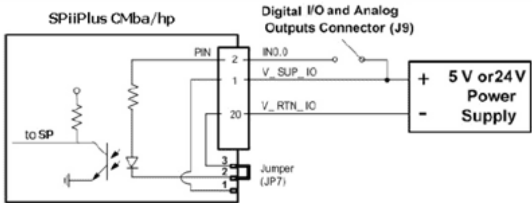
Figure 7-3. Source Digital Inputs
