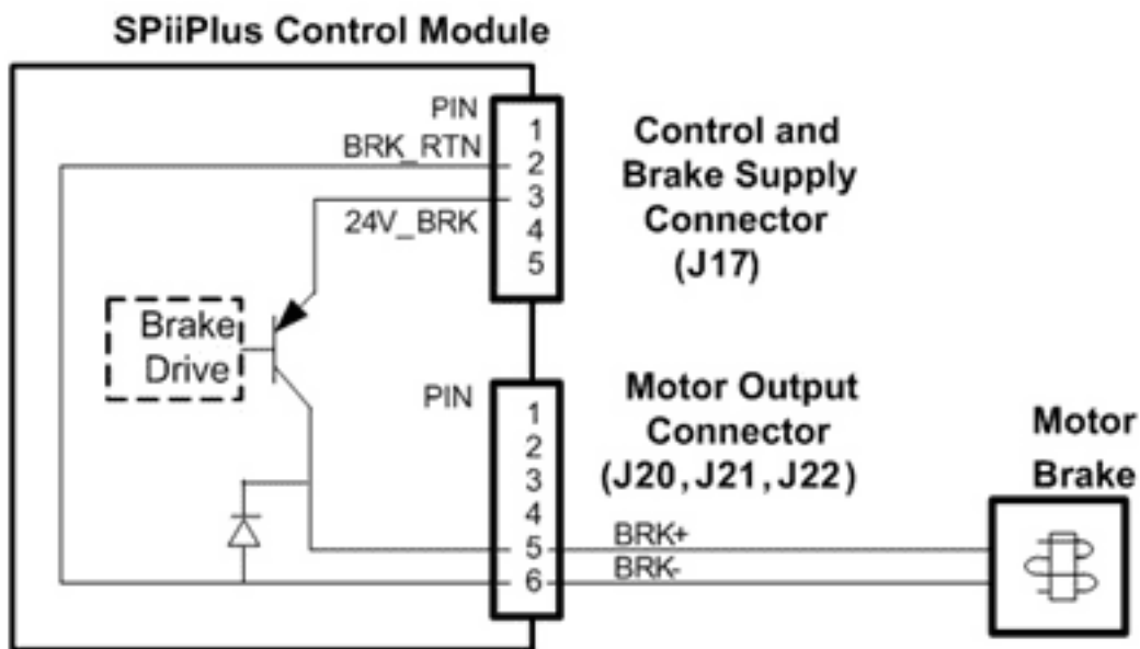
Figure 3-7. Mechanical Motor Brake
